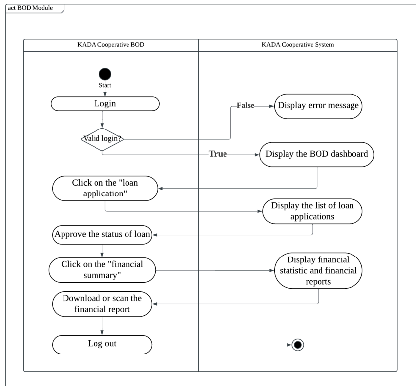
Figure 2.14 : Activity Diagram for BOD
