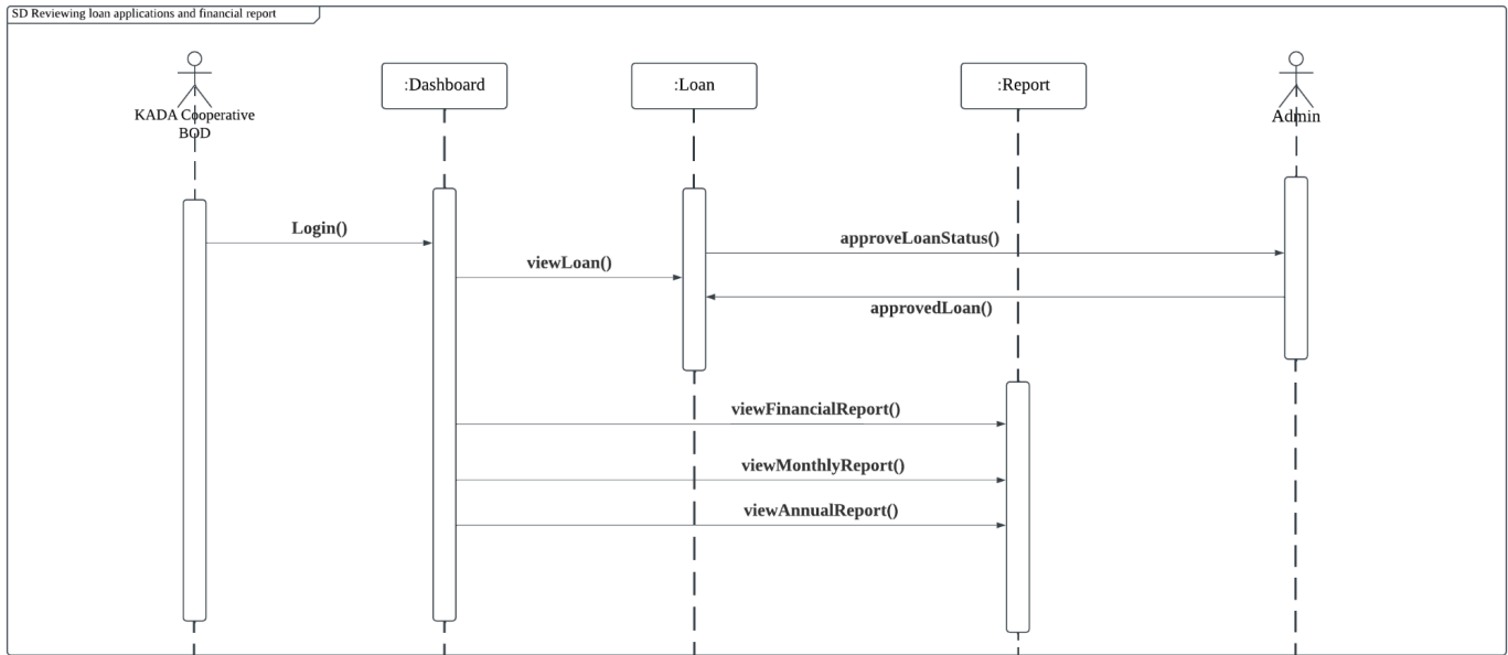
Figure 2.13 : Sequence Diagram for BOD
