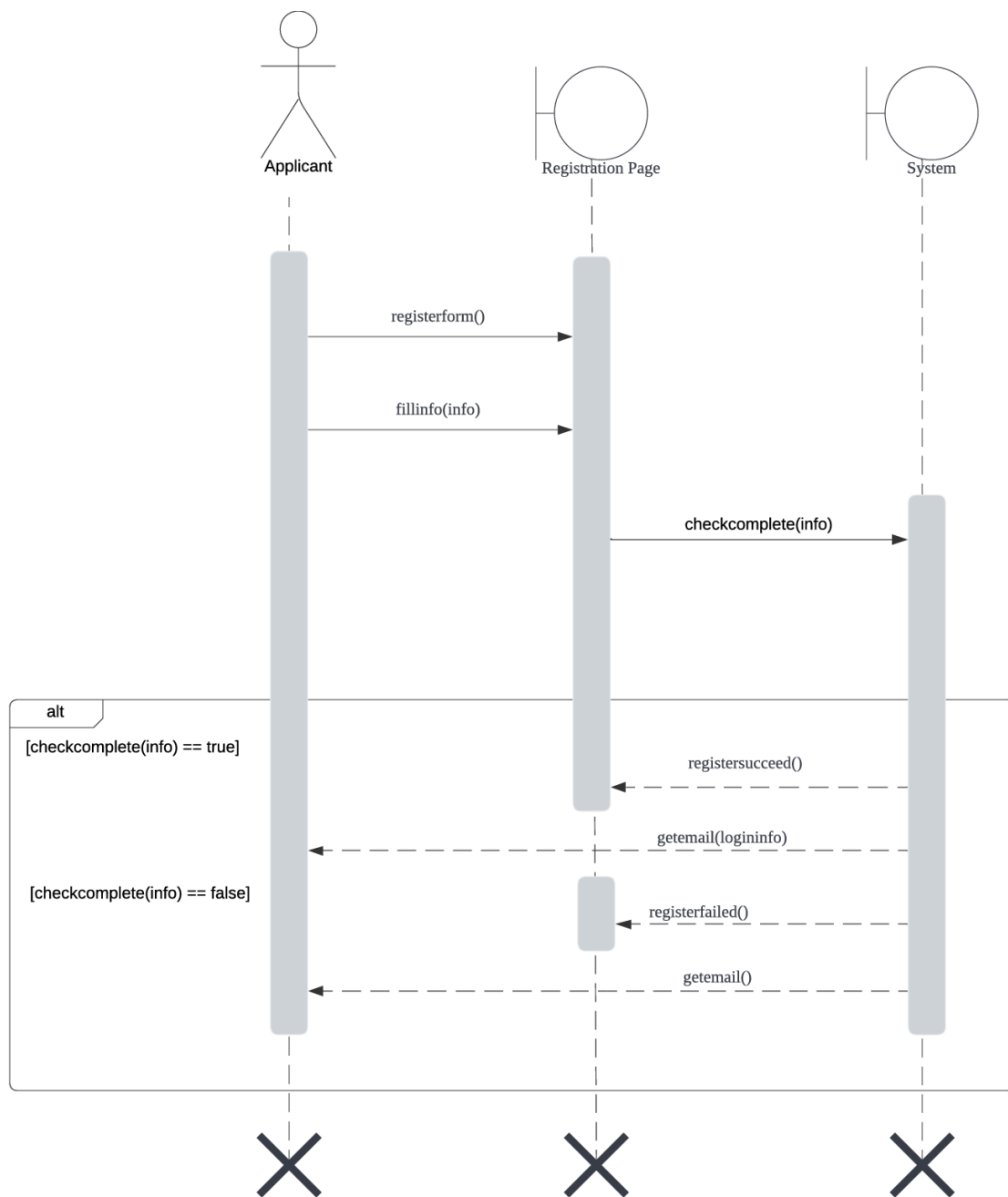
Figure 2.7 : Sequence Diagram for Applicant
