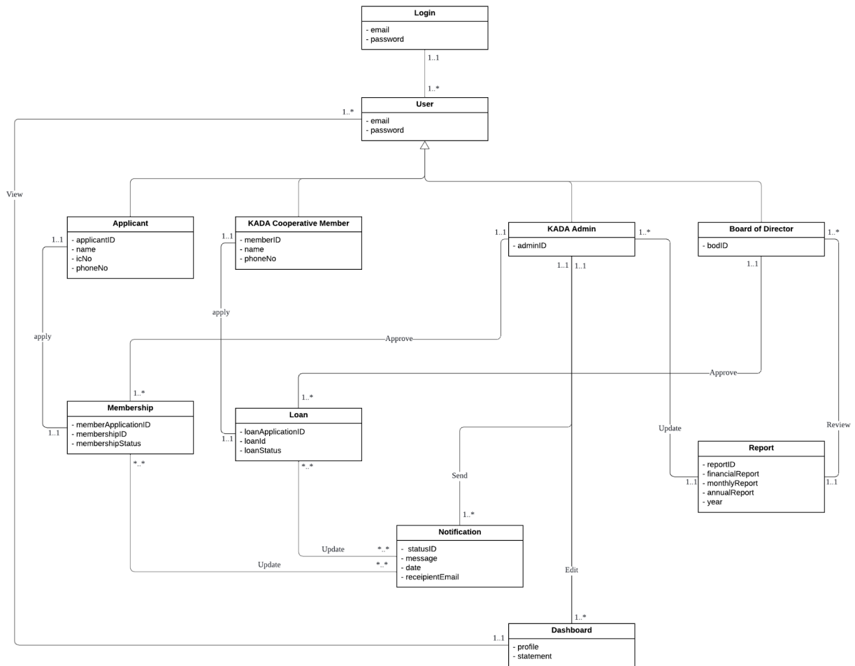
Figure 2.2 : Domain Model for KADA Cooperative System
