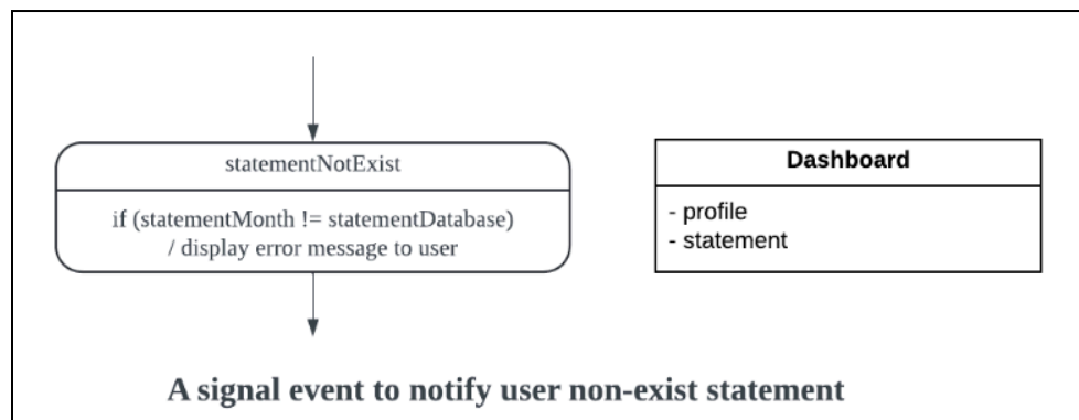
Figure 2.5 : State Machine Diagram for Dashboard
