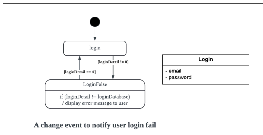
Figure 2.3 : State Machine Diagram for Login
