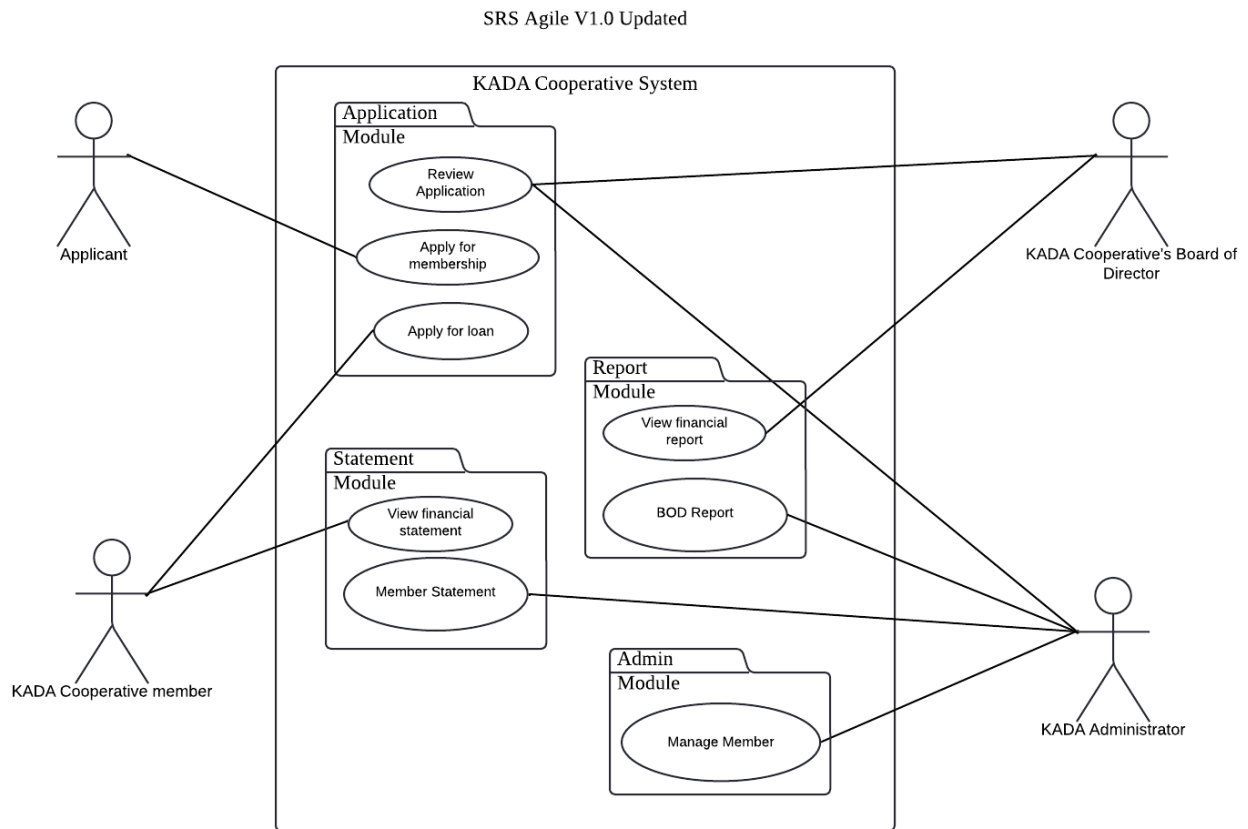
Figure 2.1: Use Case Diagram for KADA Cooperative System
