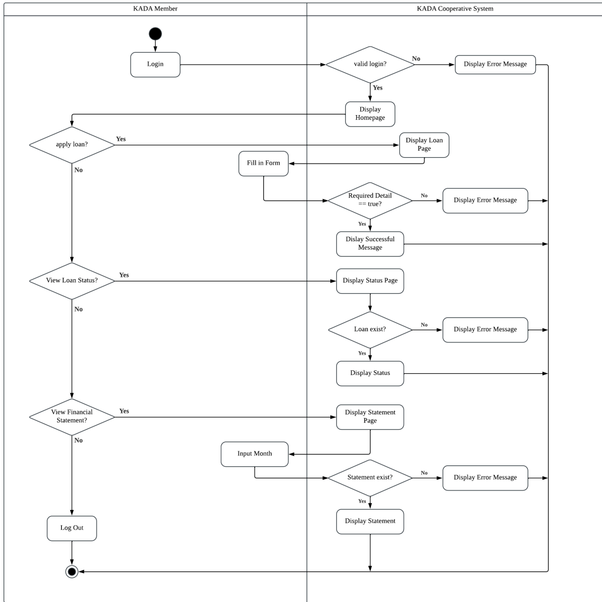
Figure 2.10 : Activity Diagram for Member
