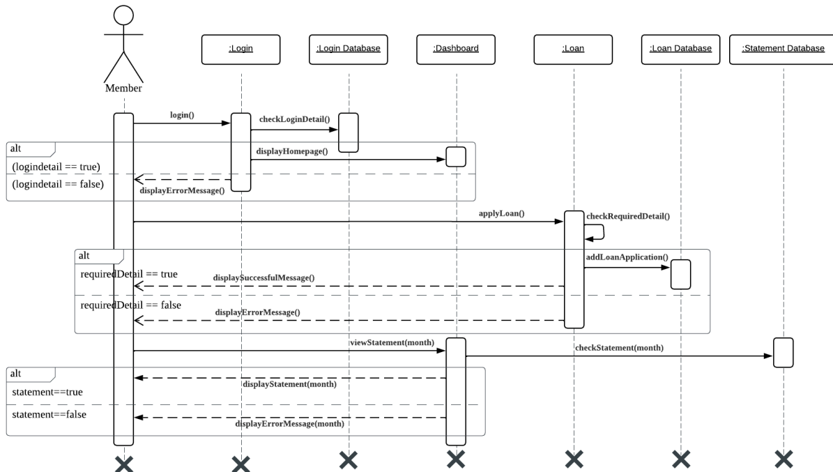
Figure 2.9: Sequence Diagram for Member
