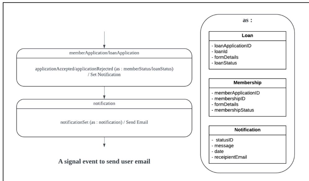
Figure 2.4 : State Machine Diagram for Membership, Loan and notification
