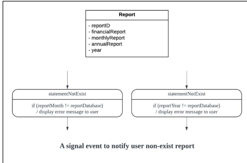
Figure 2.6 : State Machine Diagram for Report
